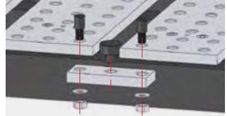
Mount the Channel Block and insert the Rest Button to create a continuous work surface over the table slot.
